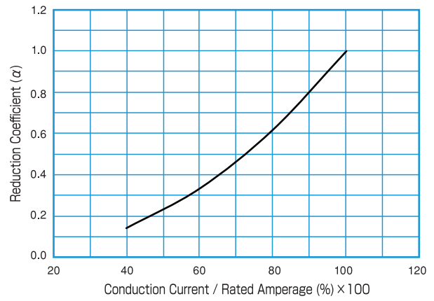
Power Loss
